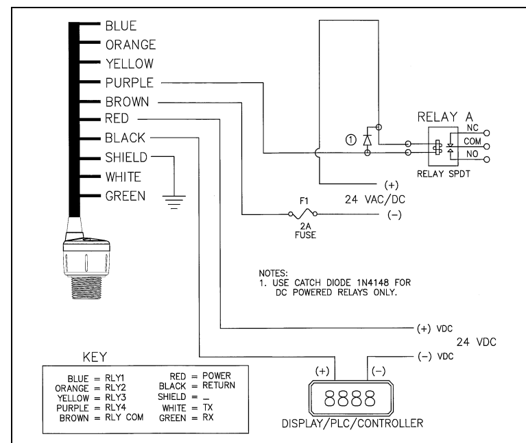
Typical Wiring Diagram Your WebCal Wiring Diagram may vary.
